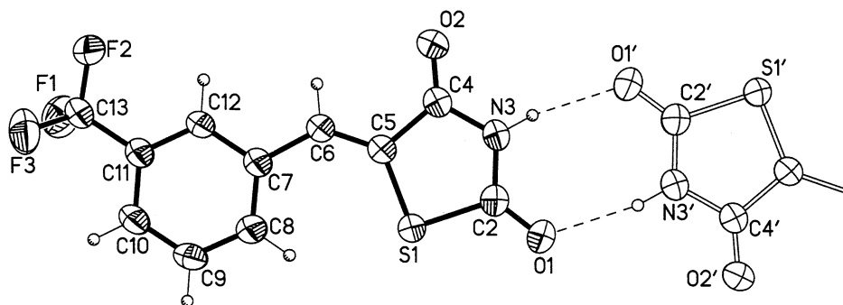
Figure 1. View of 2e on the molecule mean plane showing the atom numbering scheme. Empty atoms are of the centrosymmetric molecule at (1- x , 1- y , -1- z ) evidencing the strong H-bonds of the dimer. Thermal ellipsoids are drawn at 50% of probability, while H size is arbitrary.
